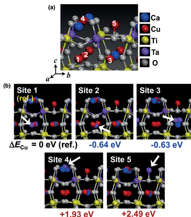
Figure 5. Set of DFT calculations showing relative stabilization of Ta in the surface Cu sites. a) Five distinct Cu sites in the surface region are denoted numerically. b) The position of Ta substituted for Site 1 was used as a reference. In contrast to Sites 1–3, \Delta E_{\text{Cu}} for Sites 4 and 5 shows significantly large positive values, proving the energetically unfavorable occupancy of Ta on the topmost surface.
